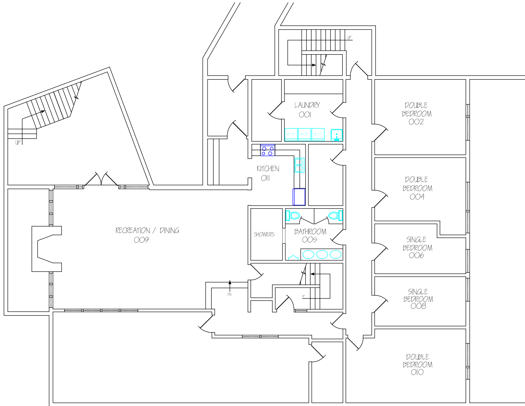
UNIT "D" GROUND FLOOR PLAN
