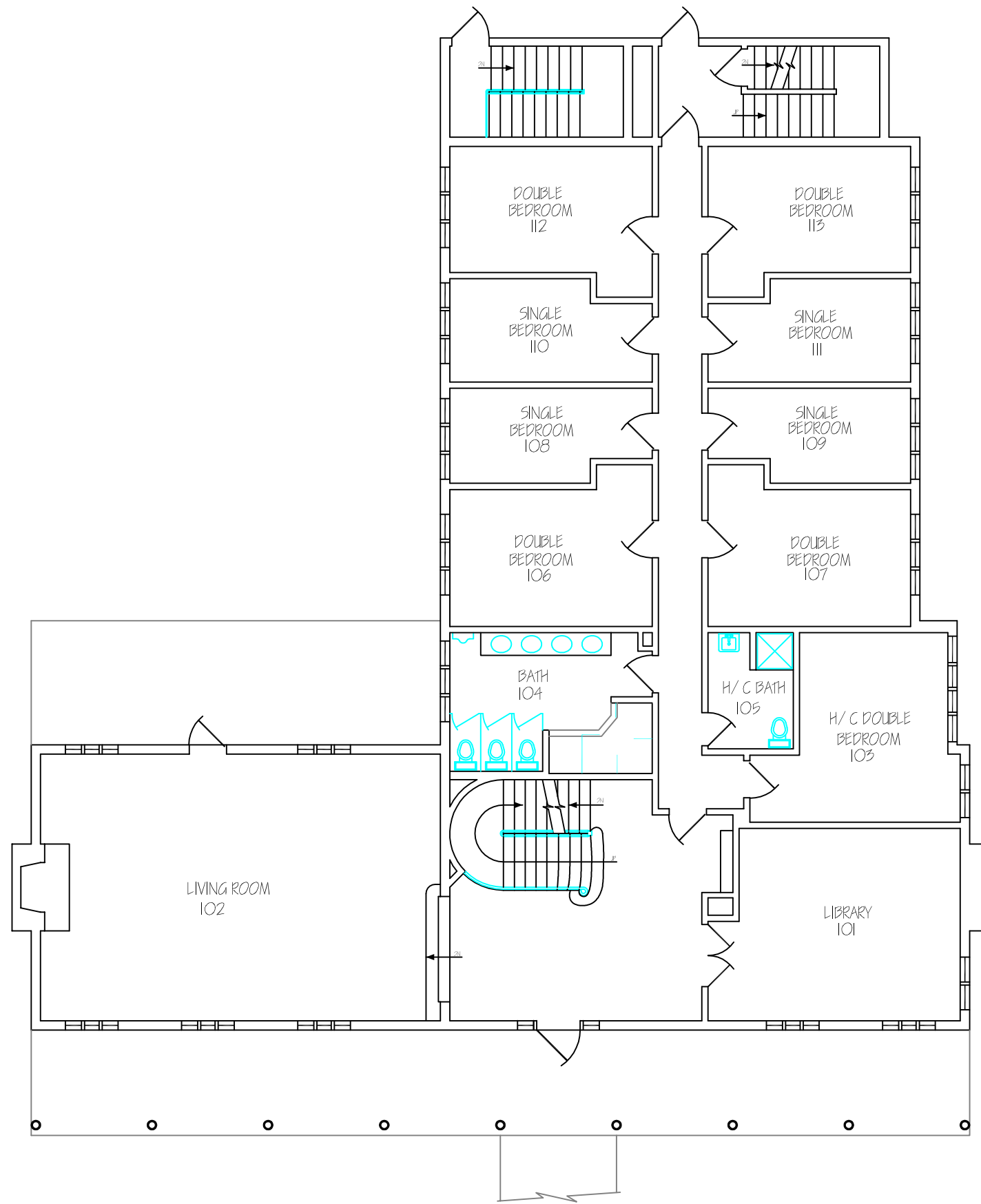
UNIT "G" FIRST FLOOR PLAN
