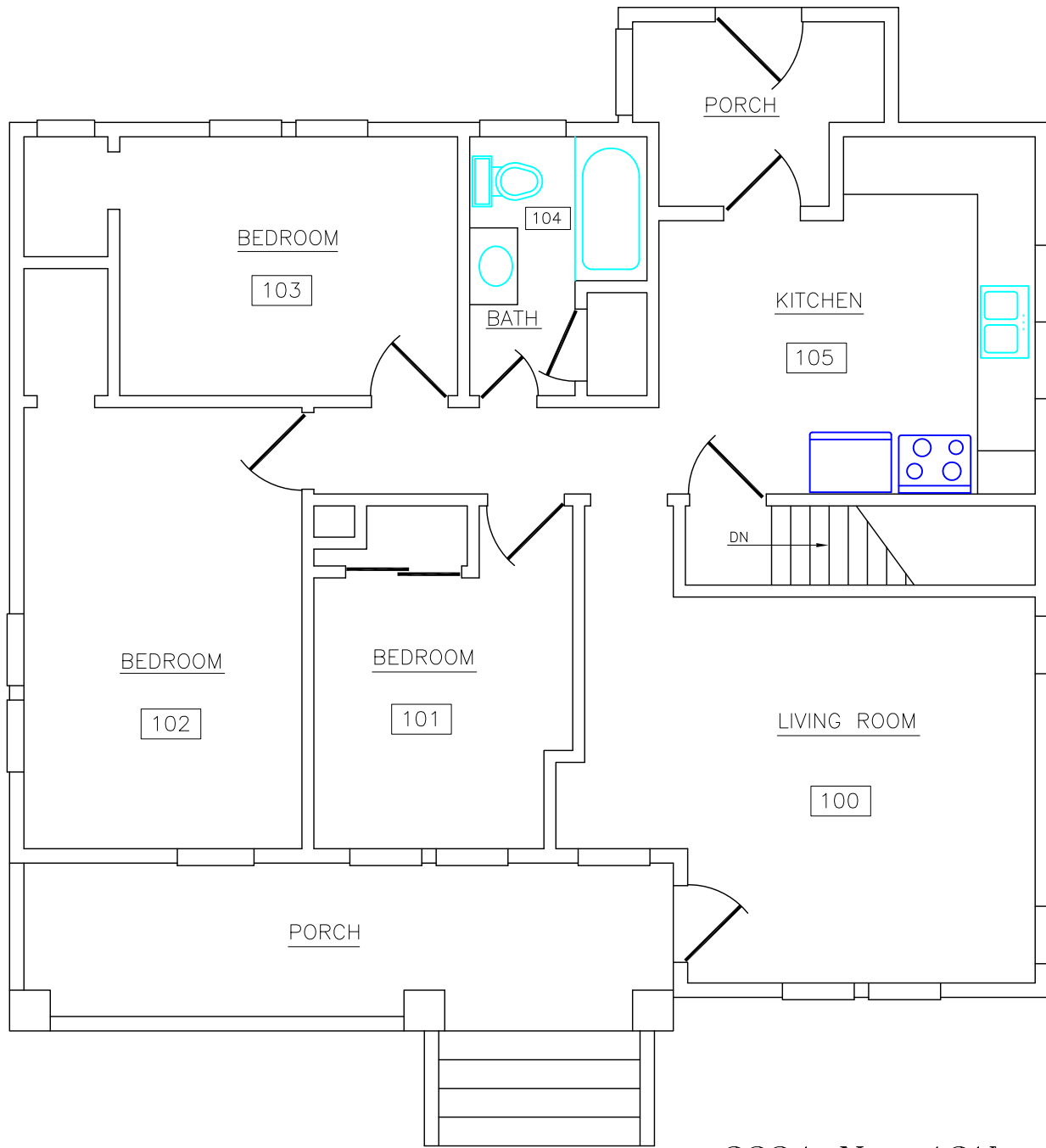
3224 No. 13th FIRST FLOOR PLAN
