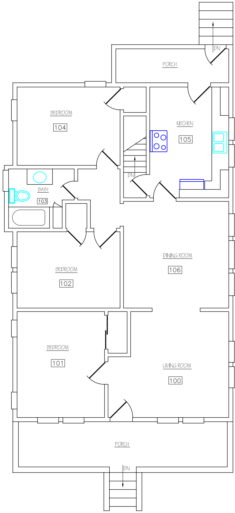
3223 No. 13th FIRST FLOOR PLAN
