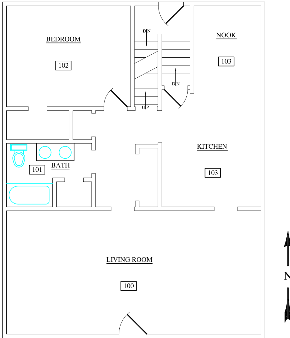
3211 No. 11th FIRST FLOOR PLAN
