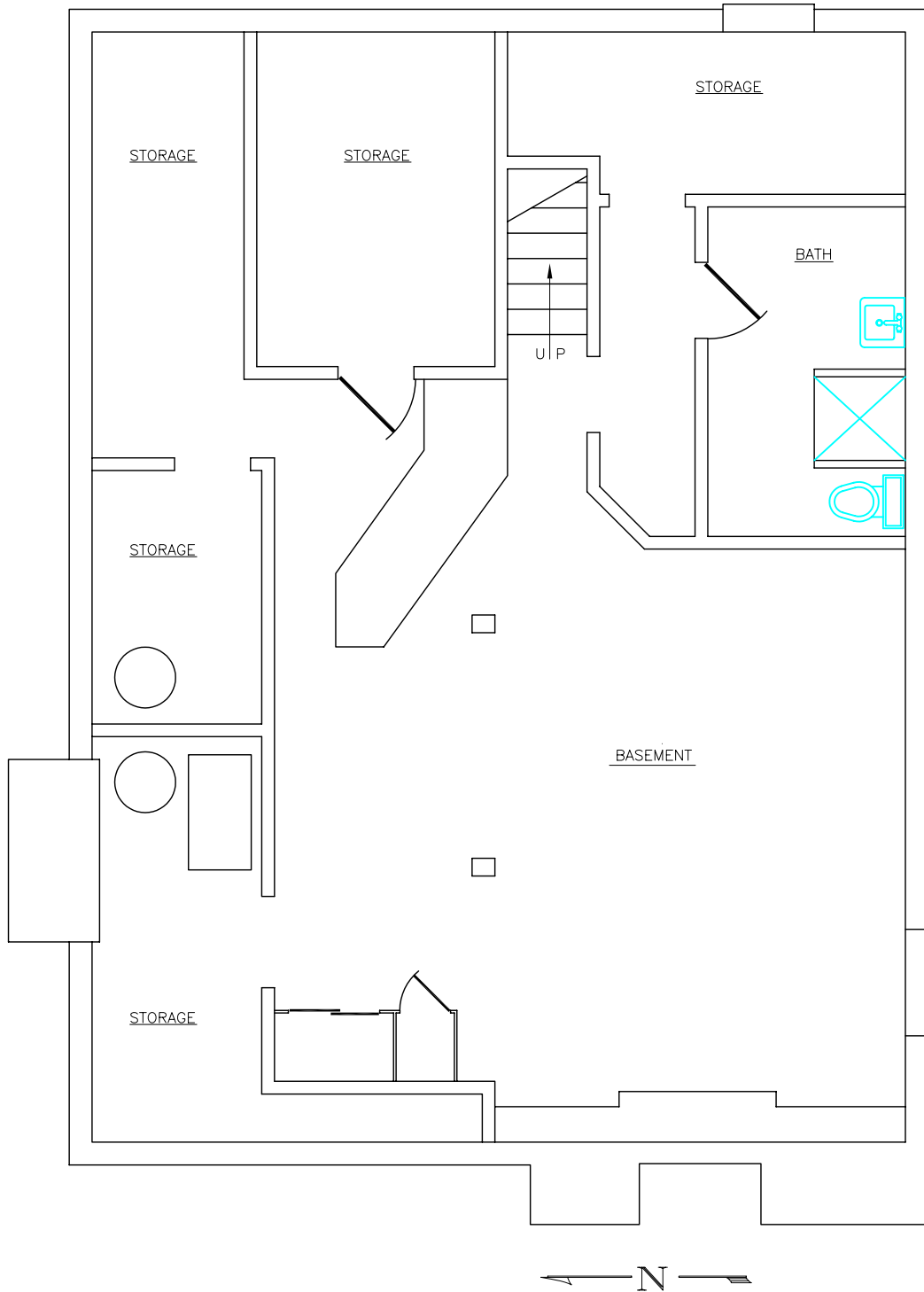
1133 No. Lawrence BASEMENT PLAN
