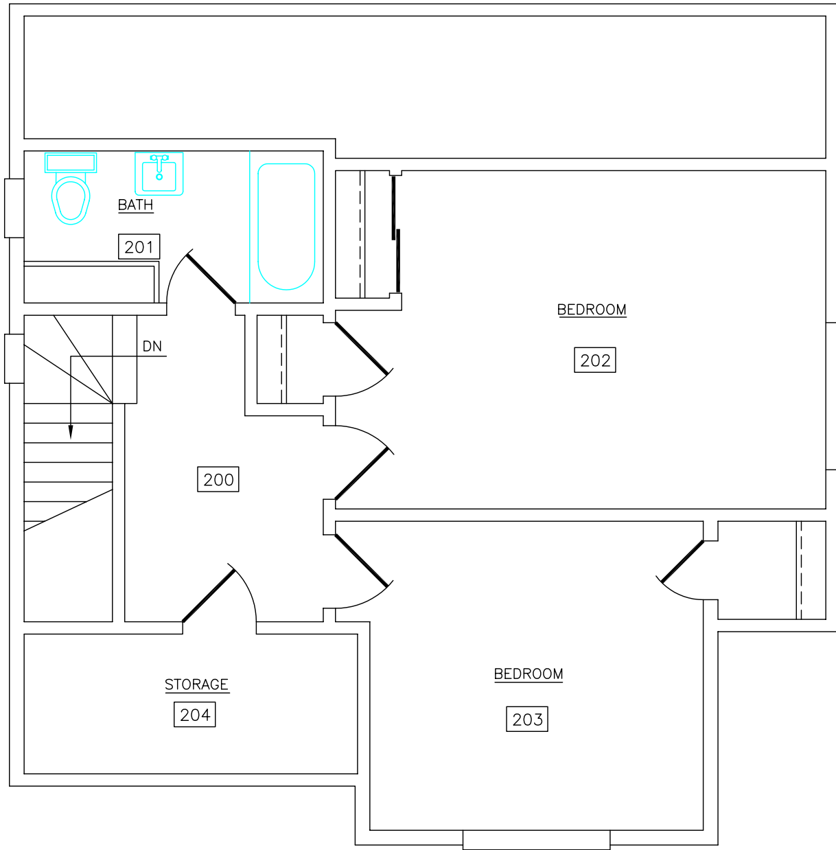
1131 No. Lawrence SECOND FLOOR PLAN
