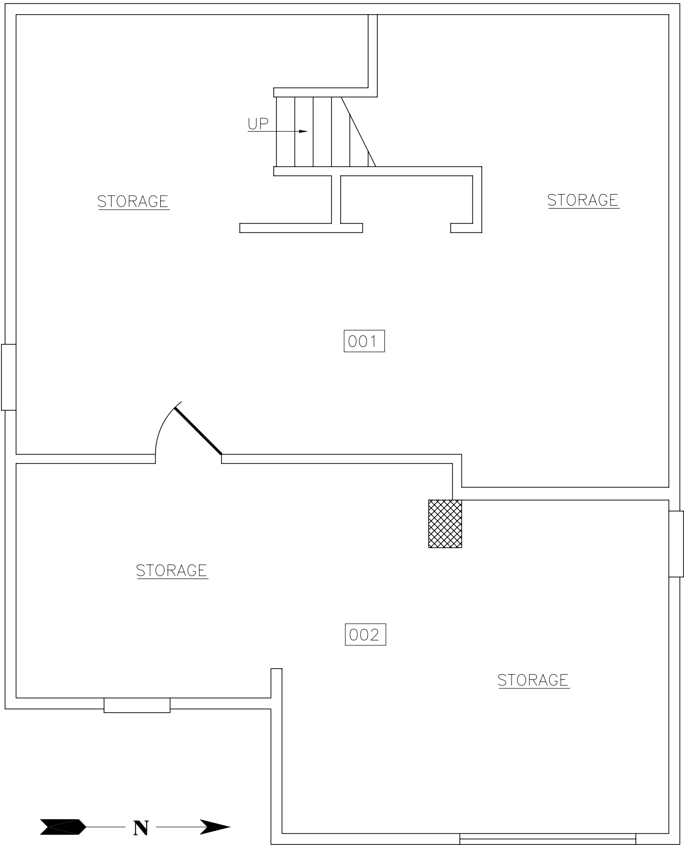
1116 No. Lawrence Basement Plan
