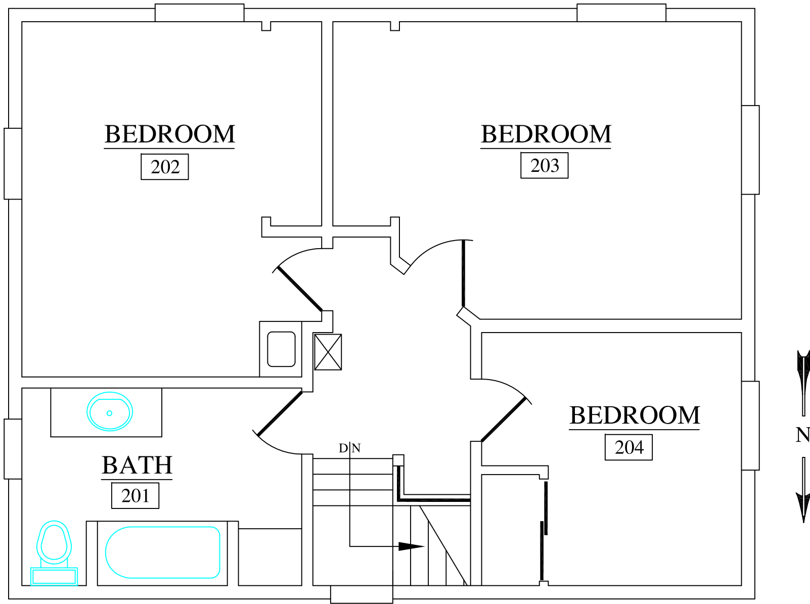
1111 No. LAWRENCE SECOND FLOOR PLAN
