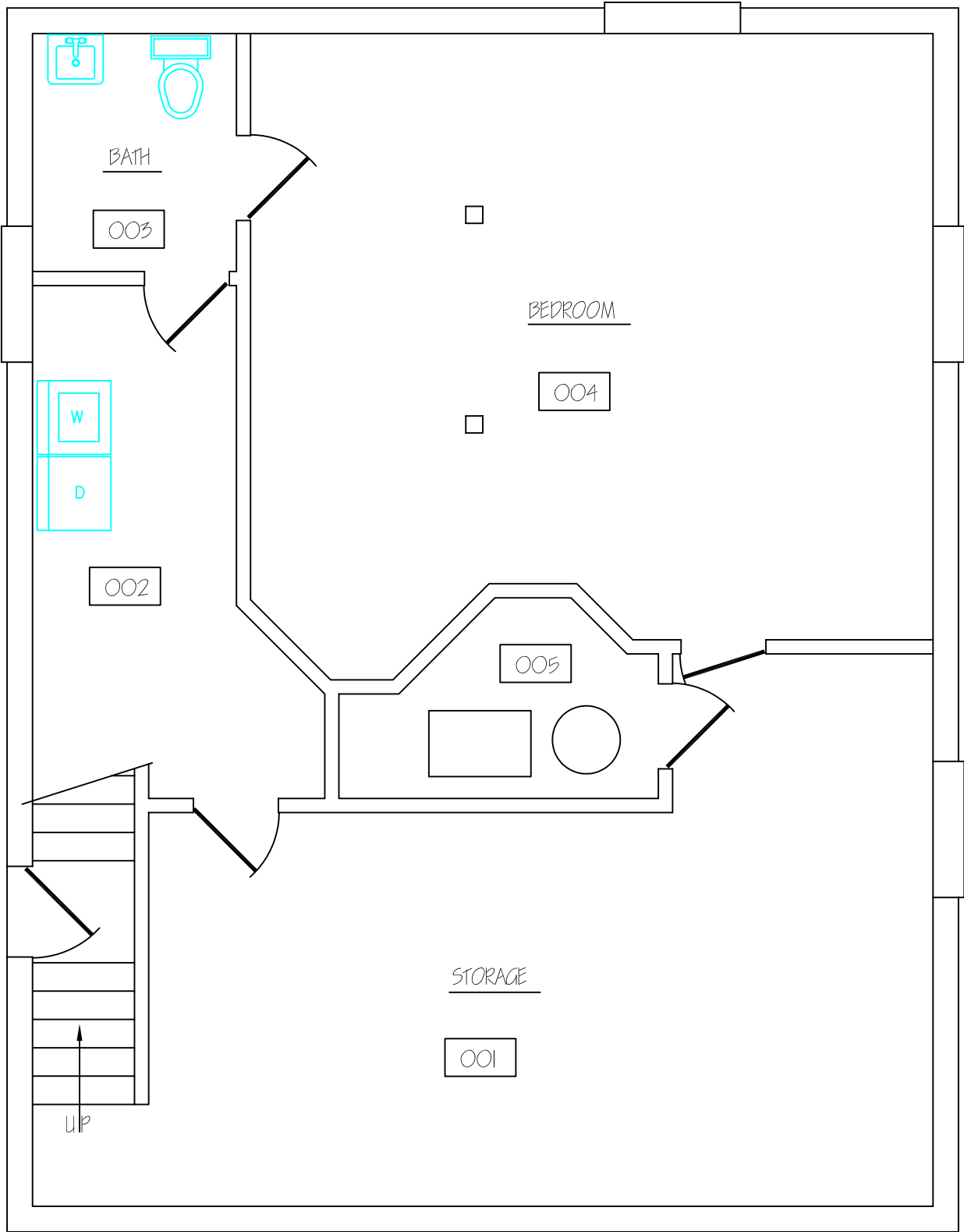
1003 No. Lawrence Basement plan
